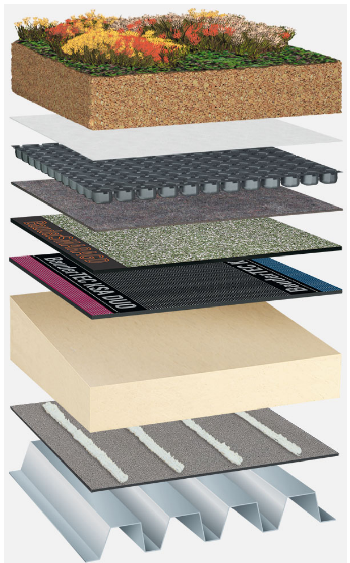
System build-up: TP_PIR-TG_S_01_G125
