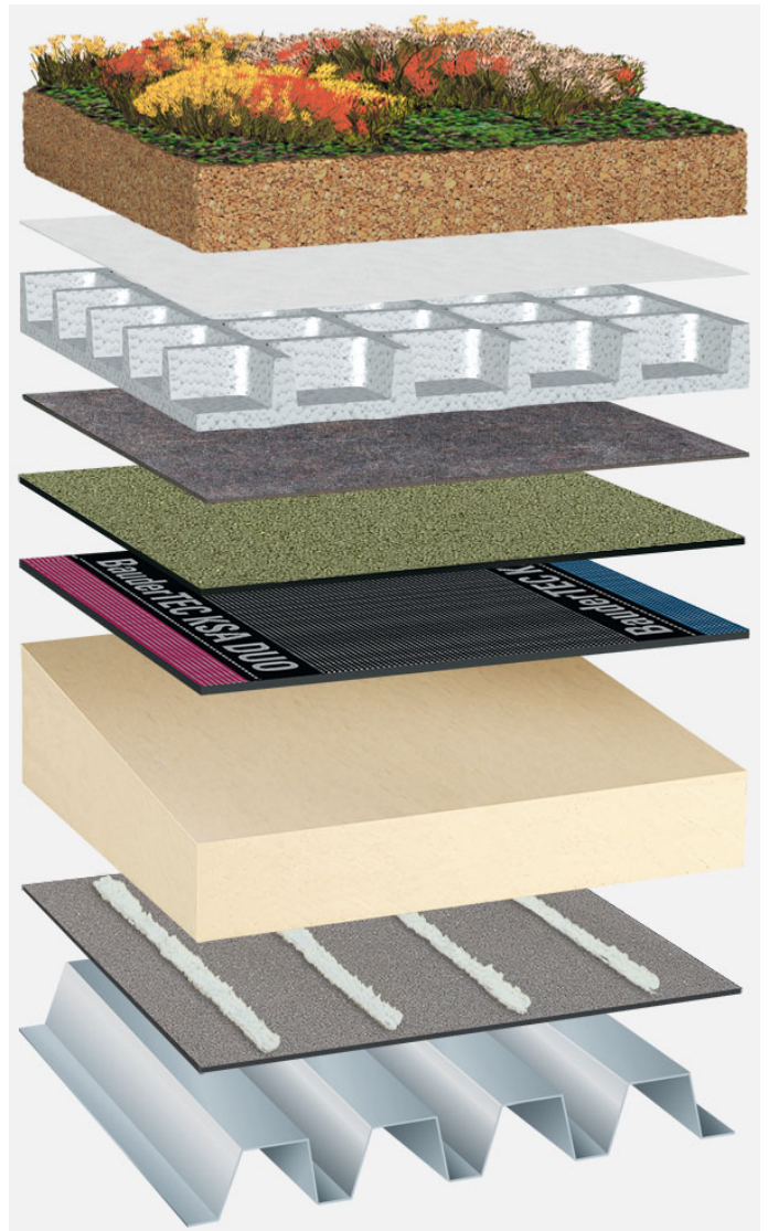
System build-up: TP_PIR-TG_P_01_G75
