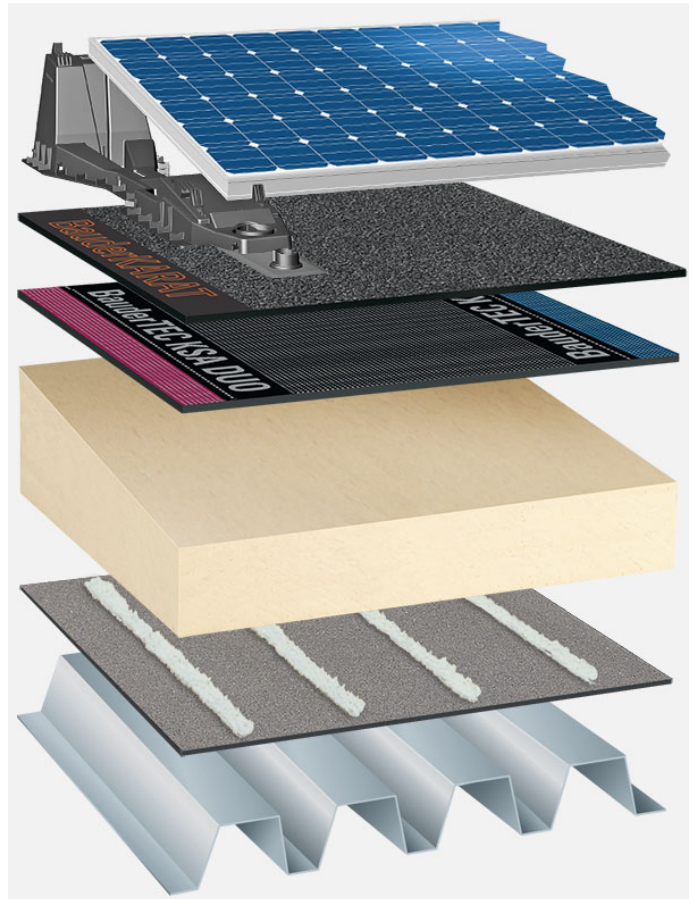
System build-up: TP_PIR-TG_K_01_PVFD
