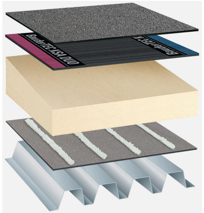
System build-up: TP_PIR-TG_B_01
