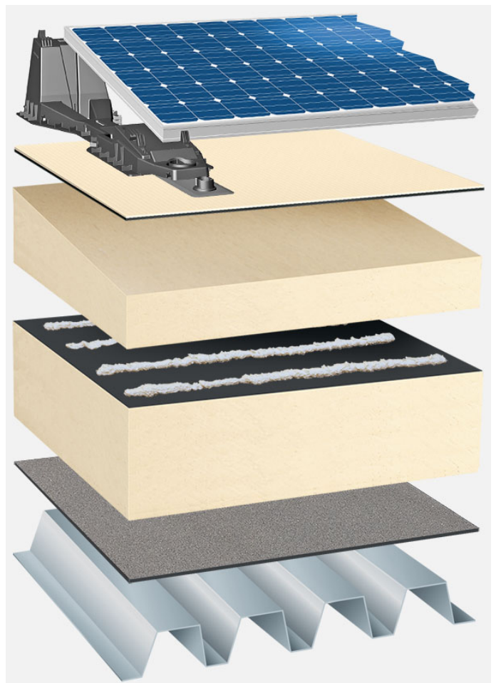
System build-up: TP_PIR-FA_PIR-TG_T_01_PVFD
