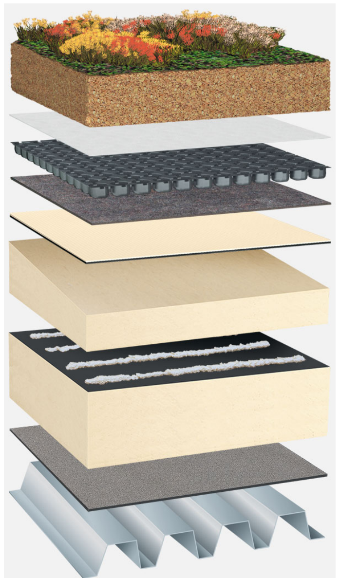
System build-up: TP_PIR-FA_PIR-TG_T_01_G125
