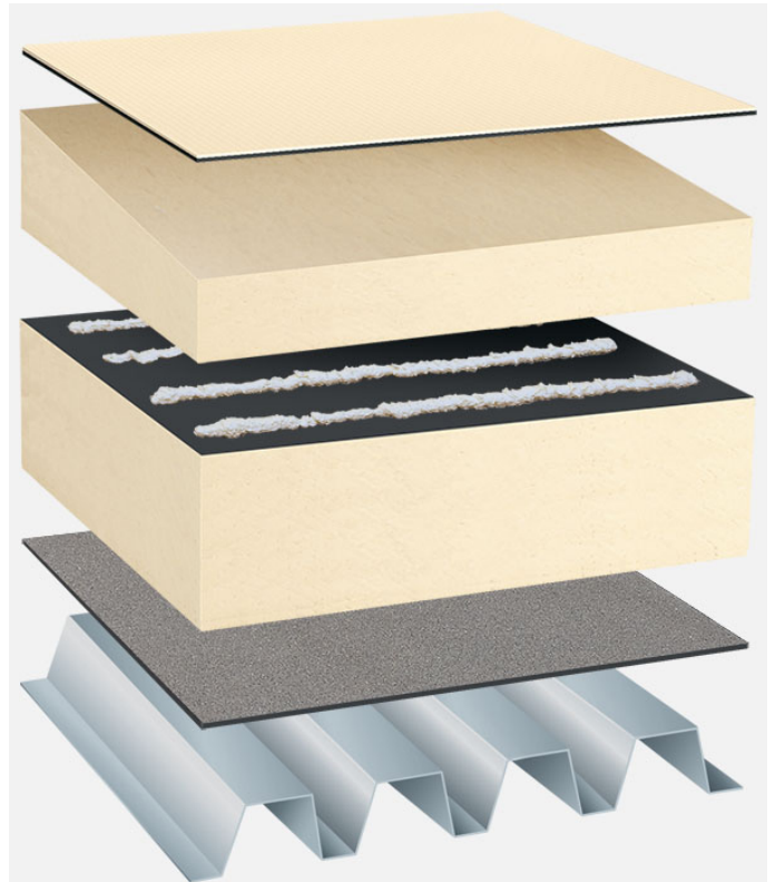
System build-up: TP_PIR-FA_PIR-TG_T_01
