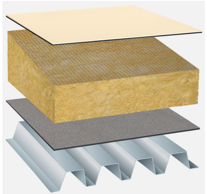
System build-up: TP_MIFA-G_T_01
