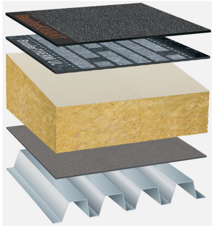
System build-up: TP_MIFA-G_K_01
