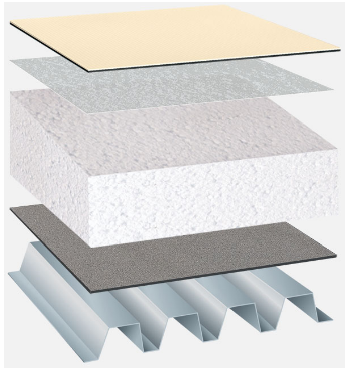
System build-up: TP_EPS-G_T_01
