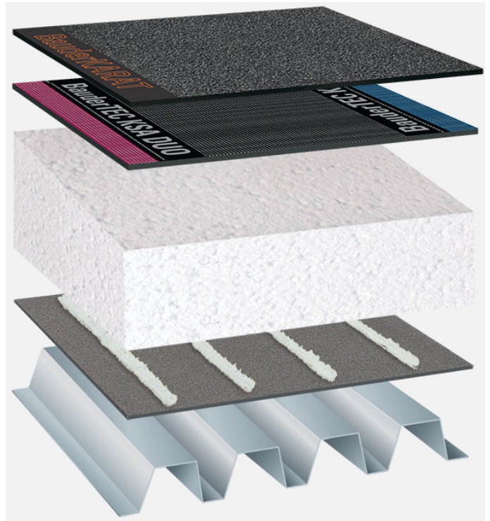
System build-up: TP_EPS-G_K_01
