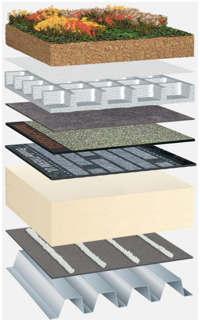
System build-up: TG_PIR-MF_S_01_G75
