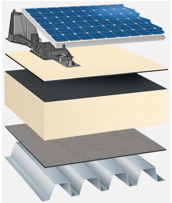
System build-up: TG_PIR-FA_T_01_PVFD
