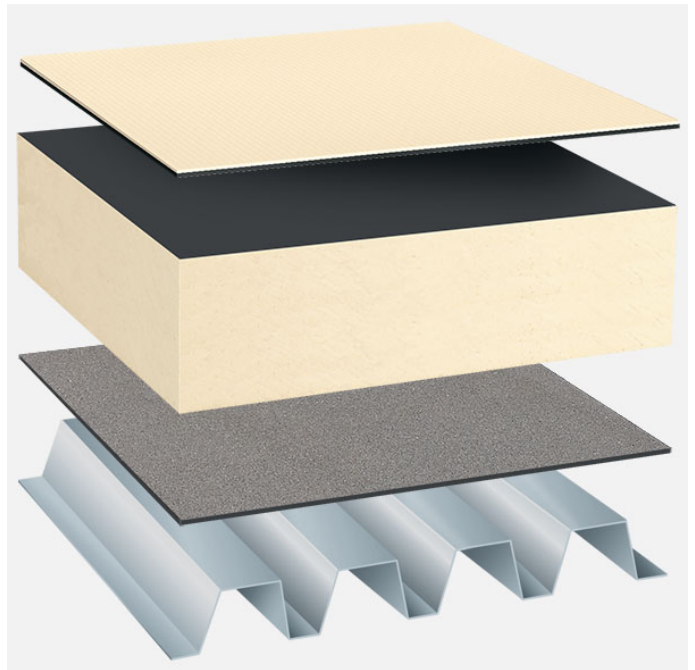
System build-up: TG_PIR-FA_T_01
