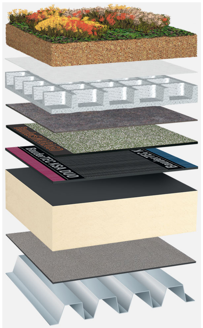
System build-up: TG_PIR-FA_S_01_G75
