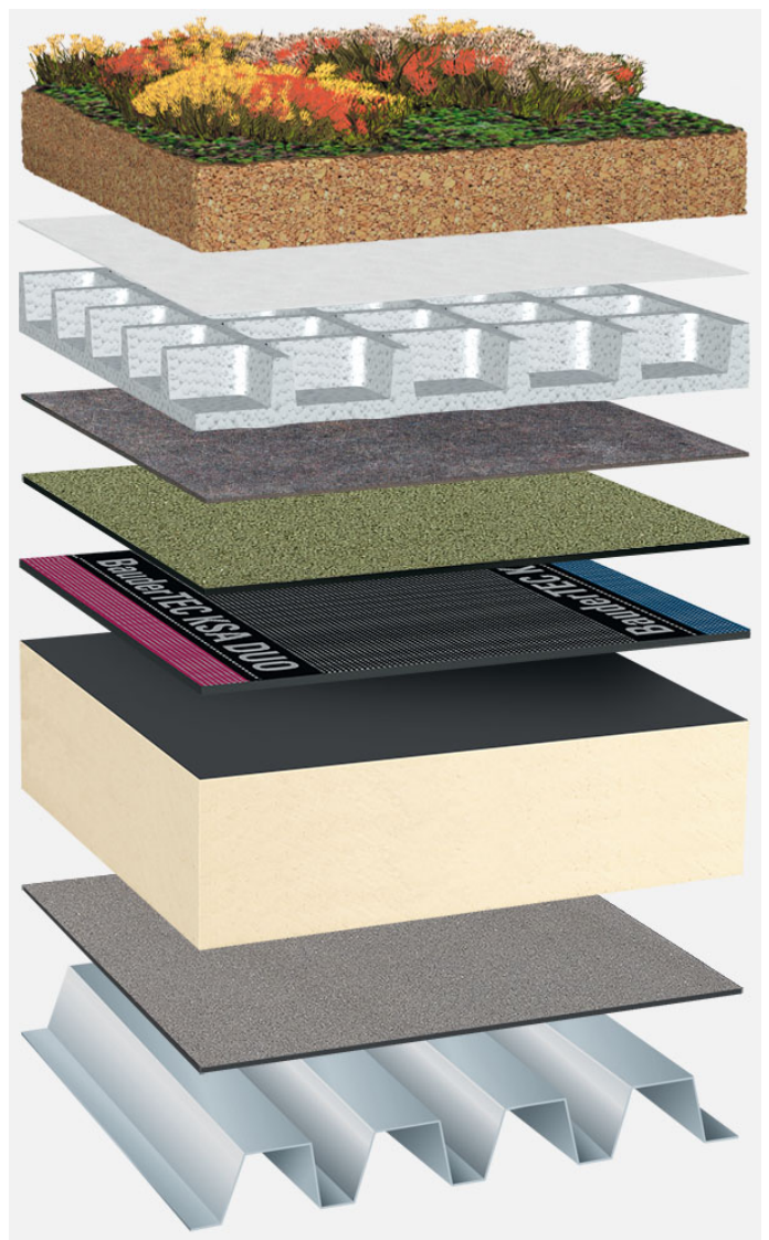
System build-up: TG_PIR-FA_P_01_G75
