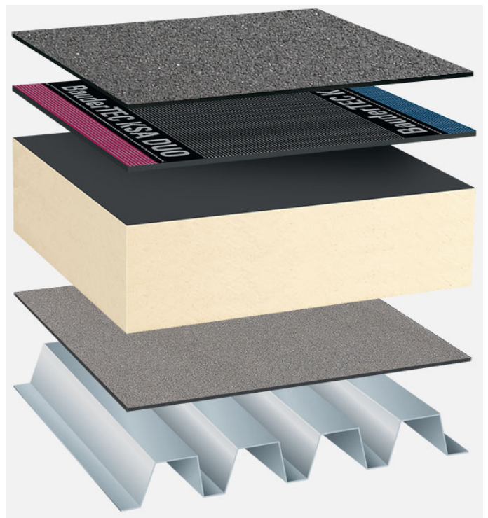
System build-up: TG_PIR-FA_B_01
