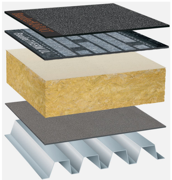
System build-up: TG_MIFA-P_K_01
