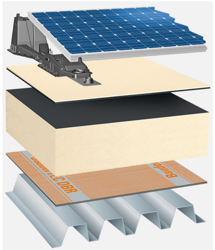
System build-up: IG_PIR-FA_T_01_PVFD
