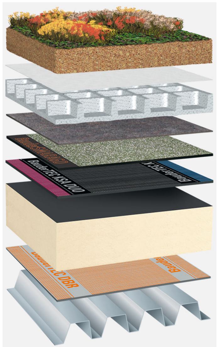
System build-up: IG_PIR-FA_S_01_G75
