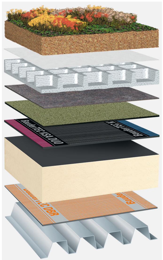
System build-up: IG_PIR-FA_P_01_G75
