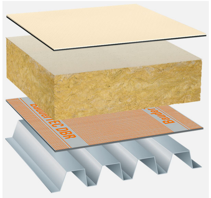
System build-up: IG_MIFA-P_T_01
