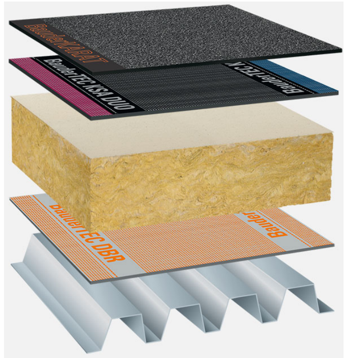
System build-up: IG_MIFA-P_K_01
