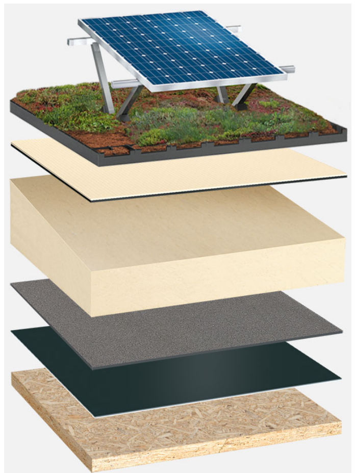
System build-up: HP_PIR-TG_T_01_PVGD
