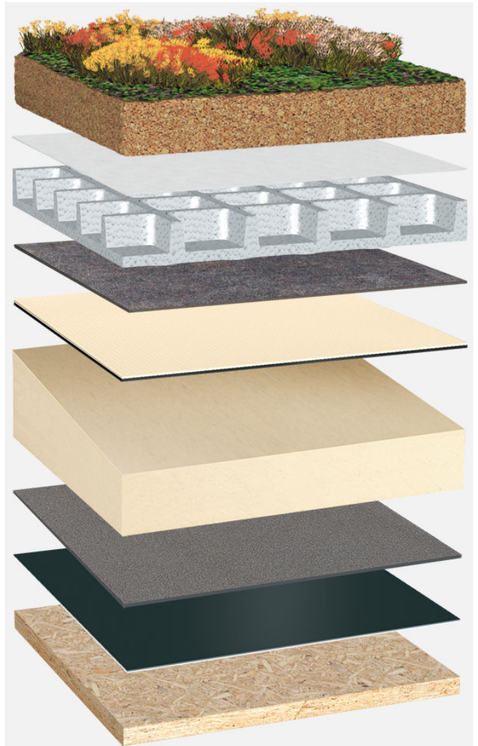
System build-up: HP_PIR-TG_T_01_G75
