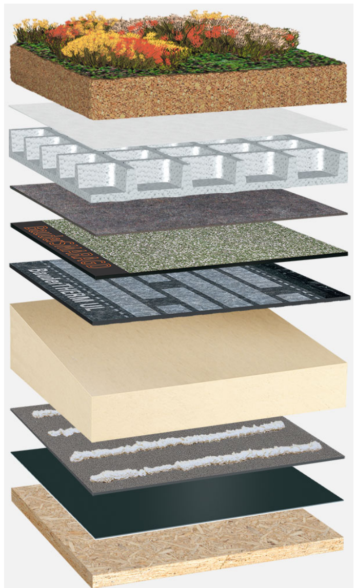
System build-up: HP_PIR-TG_S_01_G75
