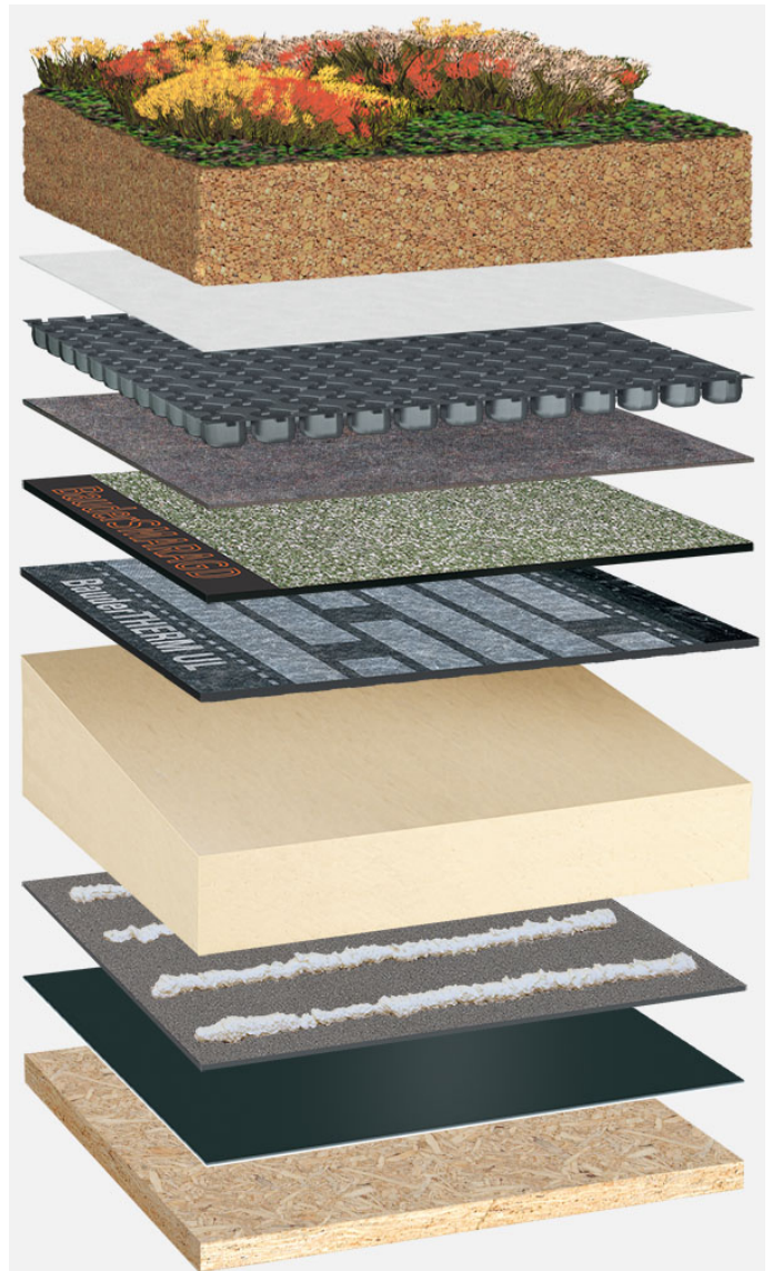
System build-up: HP_PIR-TG_S_01_G125
