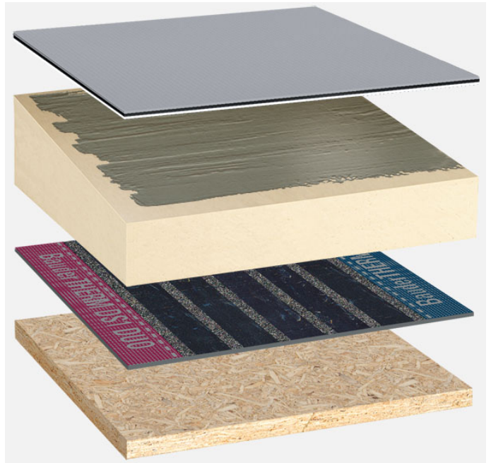
System build-up: HP_PIR-TG_SK_01
