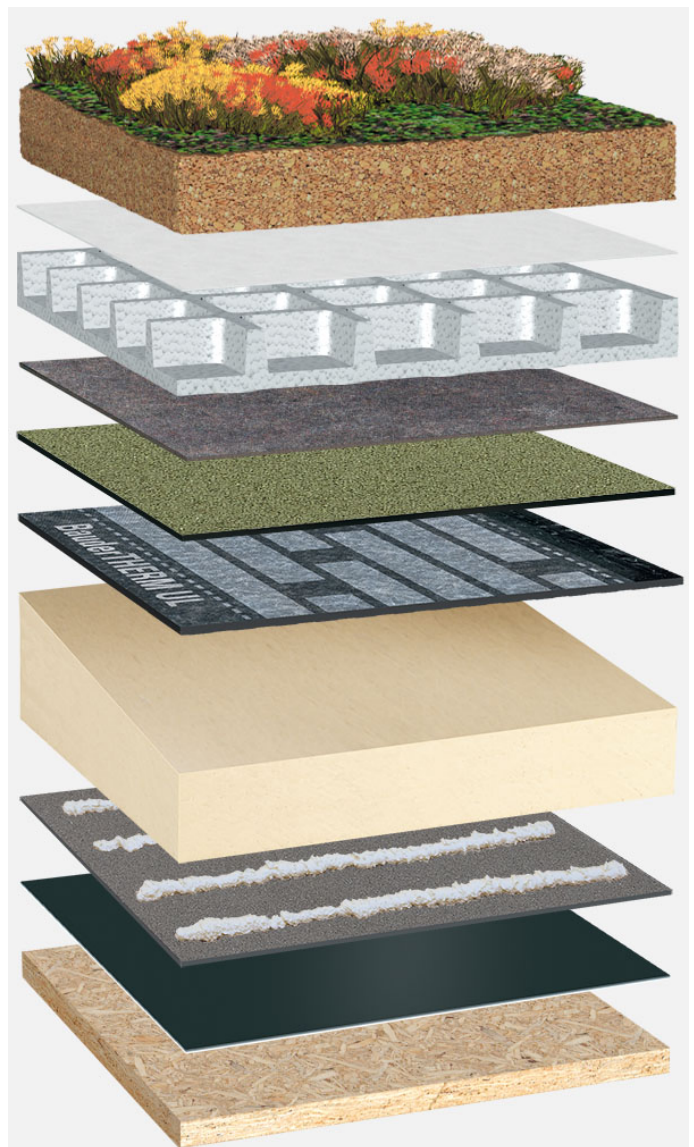
System build-up: HP_PIR-TG_P_01_G75
