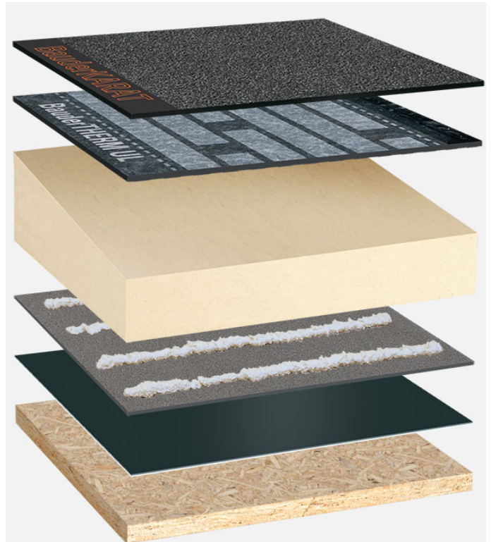
System build-up: HP_PIR-TG_K_01
