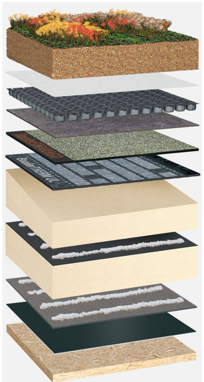
System build-up: HP_PIR-FA_PIR-TG_S_01_G125
