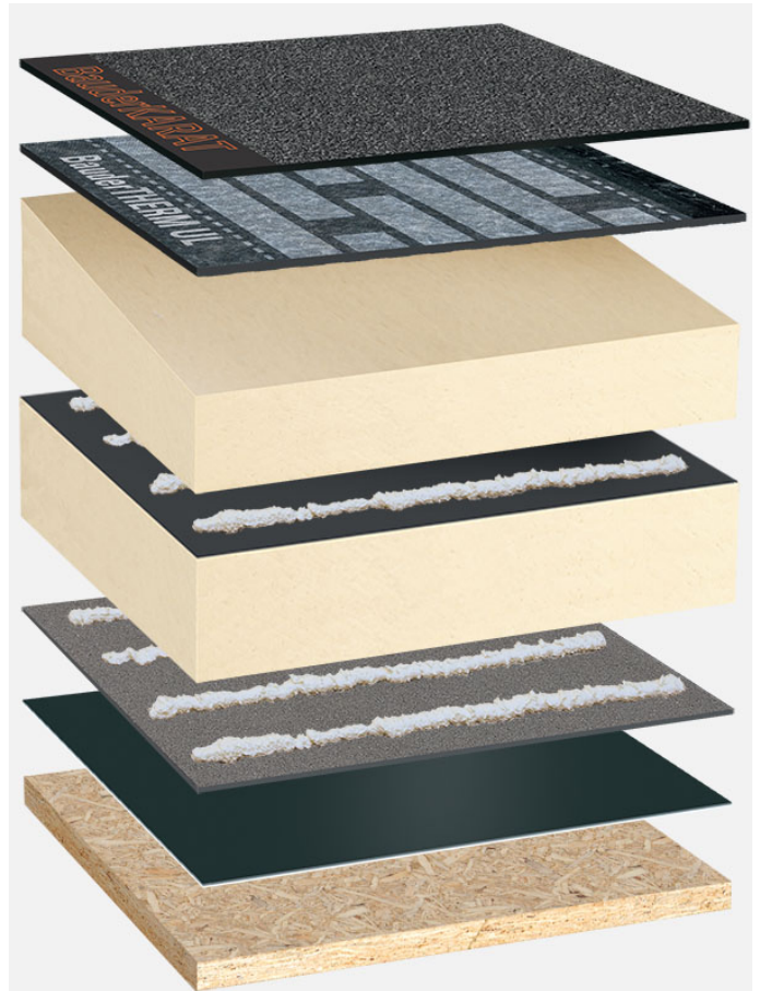
System build-up: HP_PIR-FA_PIR-TG_K_01
