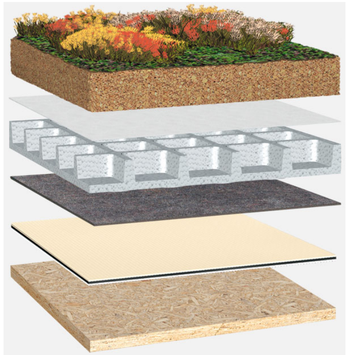
System build-up: HG_TV_01_G75
