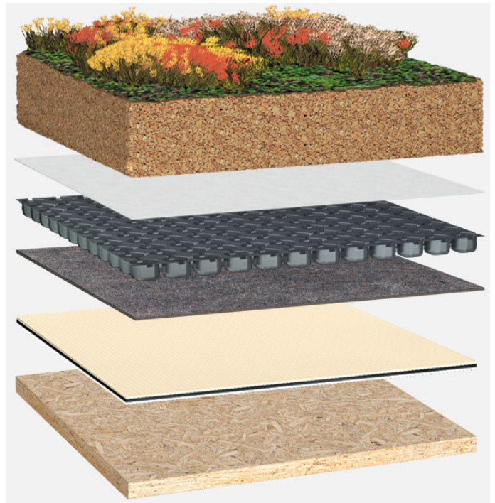
System build-up: HG_TV_01_G125
