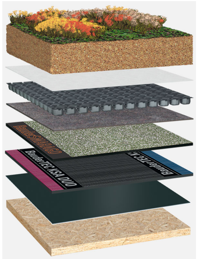
System build-up: HG_S_02_G125
