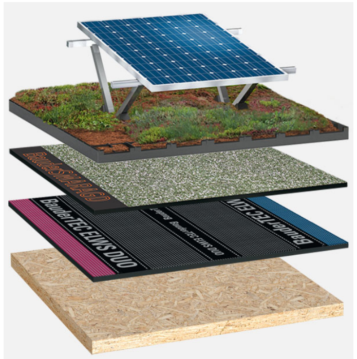
System build-up: HG_S_01_PVGD
