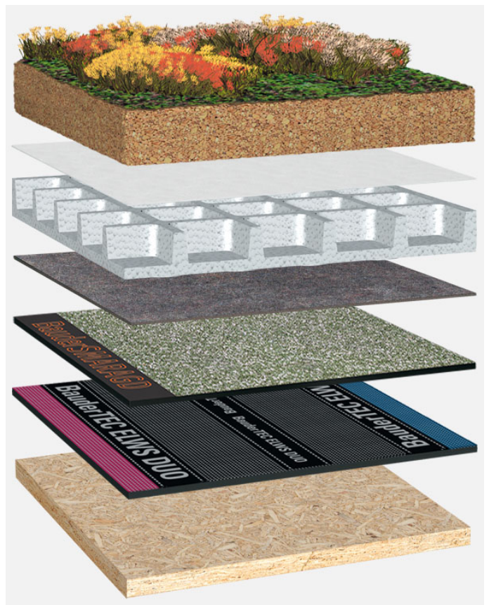
System build-up: HG_S_01_G75
