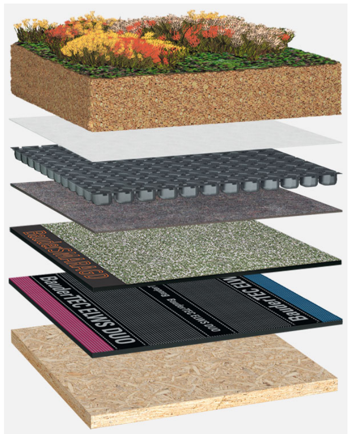
System build-up: HG_S_01_G125
