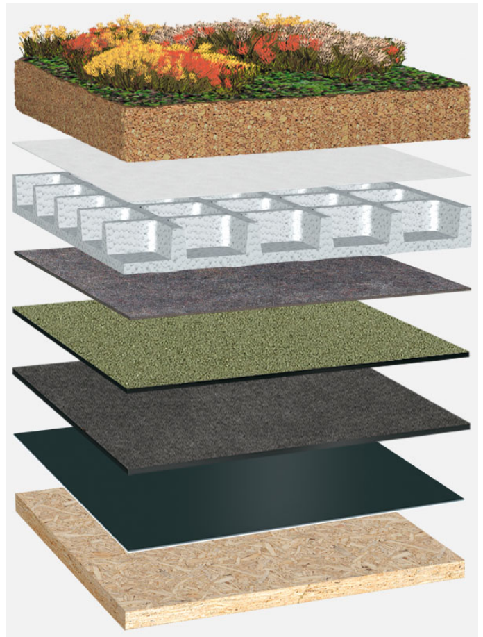
System build-up: HG_P_01_G75
