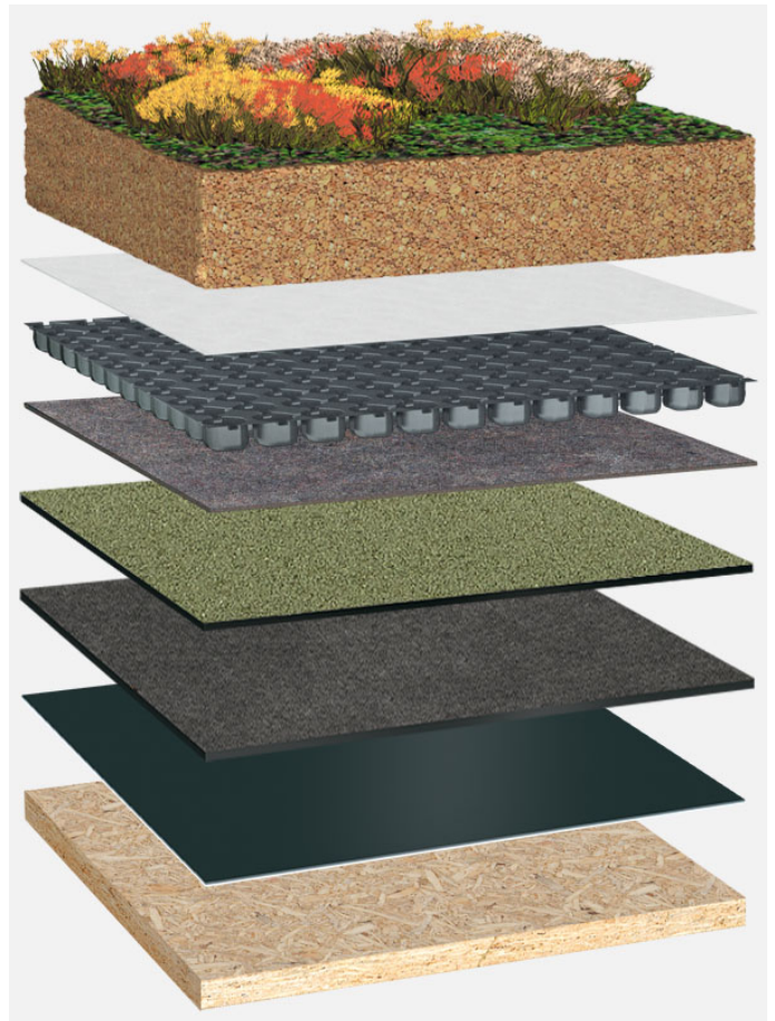
System build-up: HG_P_01_G125
