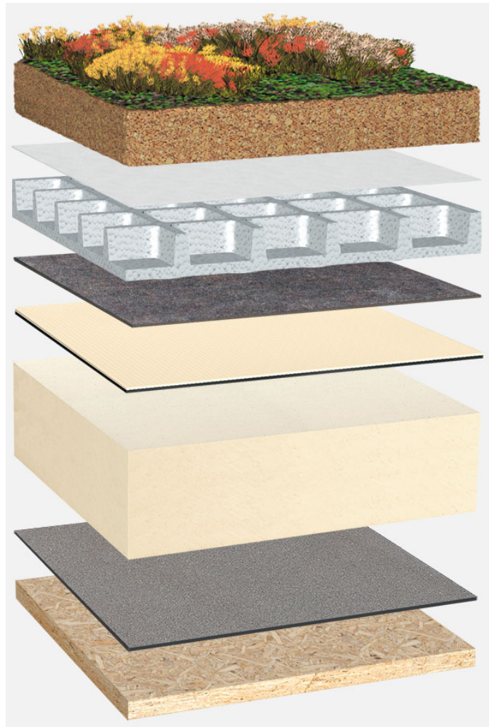
System build-up: HG_PIR-MF_T_01_G75
