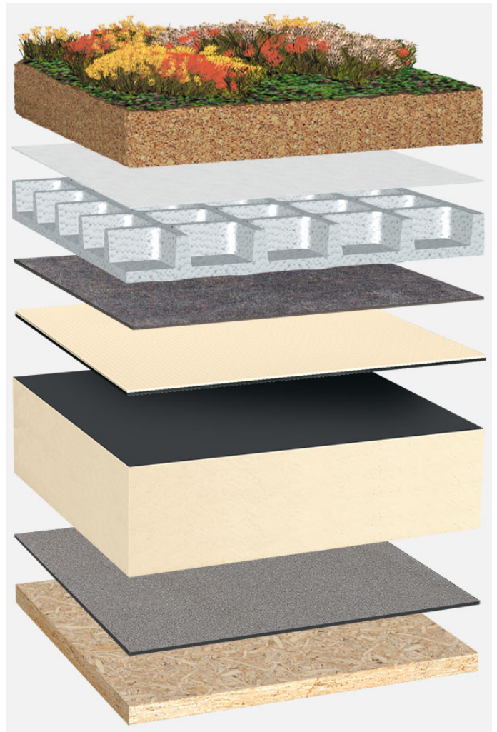
System build-up: HG_PIR-FA_T_01_G75
