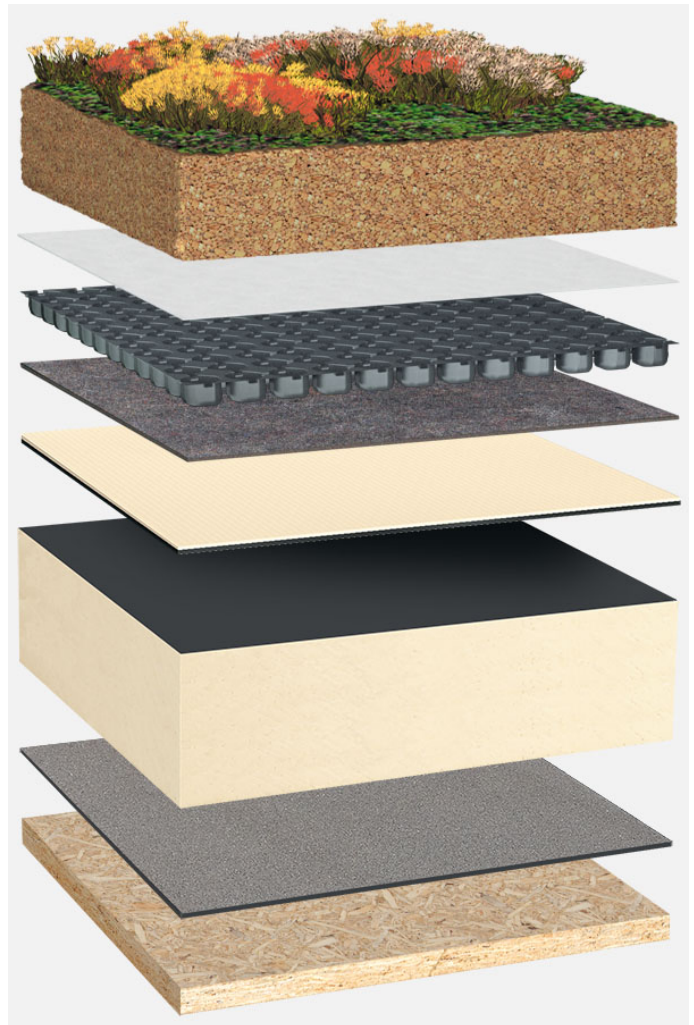
System build-up: HG_PIR-FA_T_01_G125
