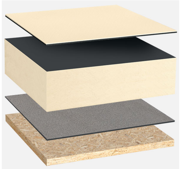
System build-up: HG_PIR-FA_T_01
