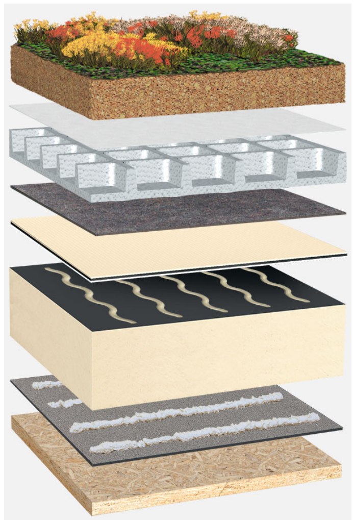
System build-up: HG_PIR-FA_TV_01_G75
