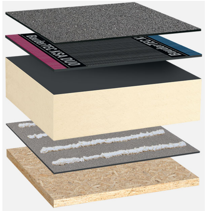
System build-up: HG_PIR-FA_B_01
