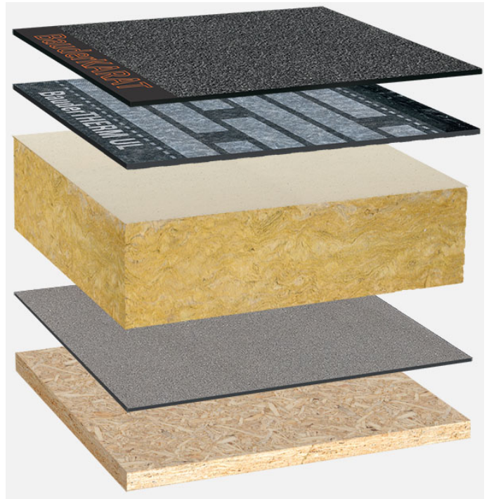
System build-up: HG_MIFA-P_K_01
