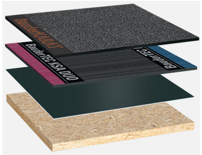
System build-up: HG_K_02
