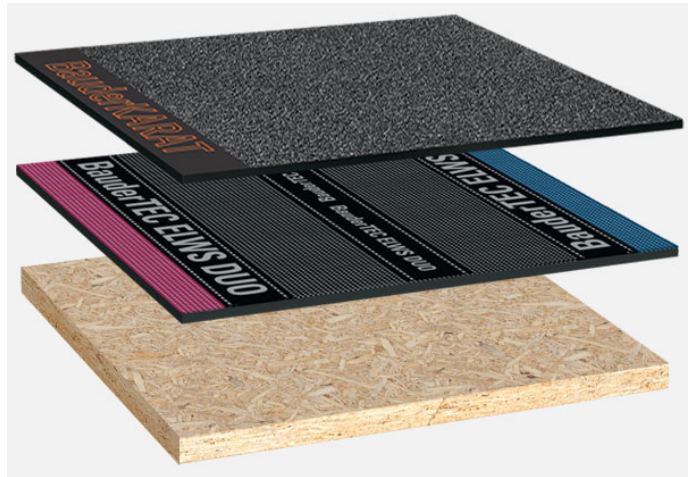
System build-up: HG_K_01
