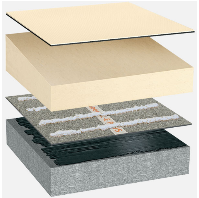
System build-up: BP_PIR-TG_T_02
